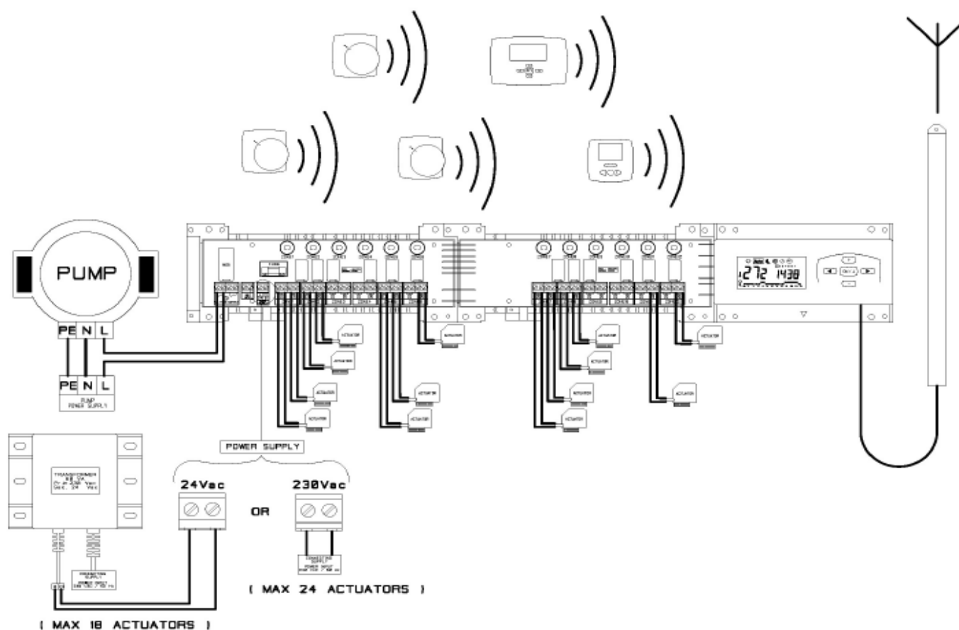
WIRING ASSEMBLY DIAGRAM
